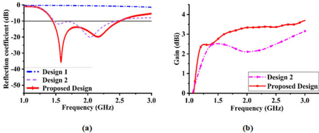
Figure 2. Antenna Performance in Each Step of Try and Error Method; (a) Reflection Coefficient; (b) Gain.
