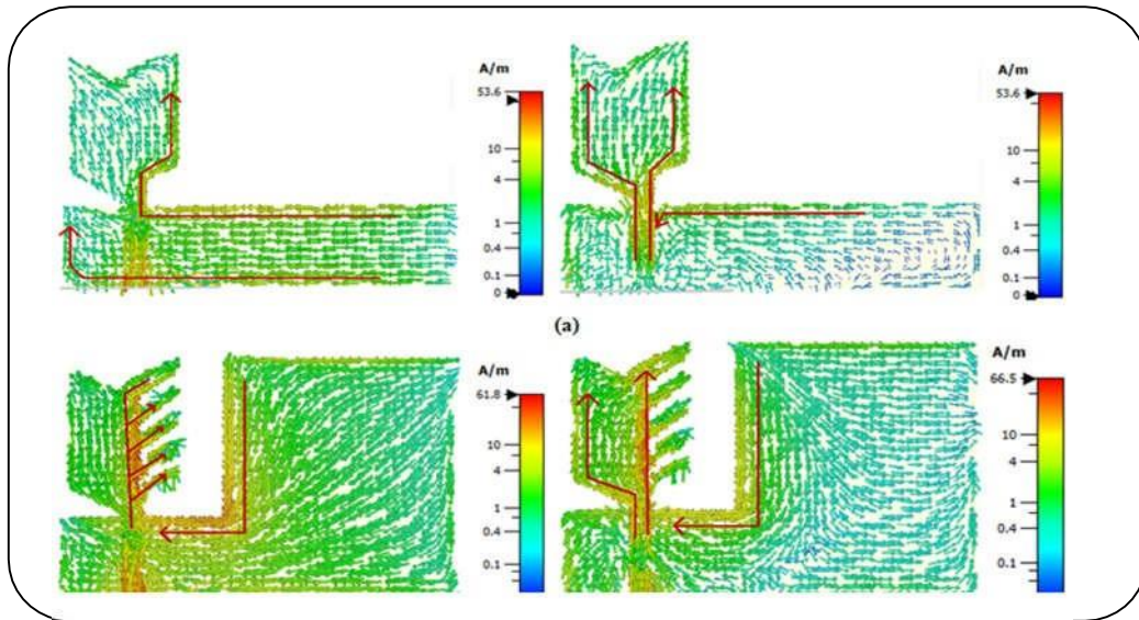
Figure 3. Surface current allocation for different step of design evolution at multiple frequency point; (a) Design 2 at 1.58 GHz and 2.17 GHz, (b) Final design at 1.58 GHz and 2.17 GHz.
