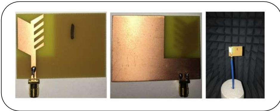
Figure 4. Fabricated Prototype and Anechoic Chamber Measurement.
