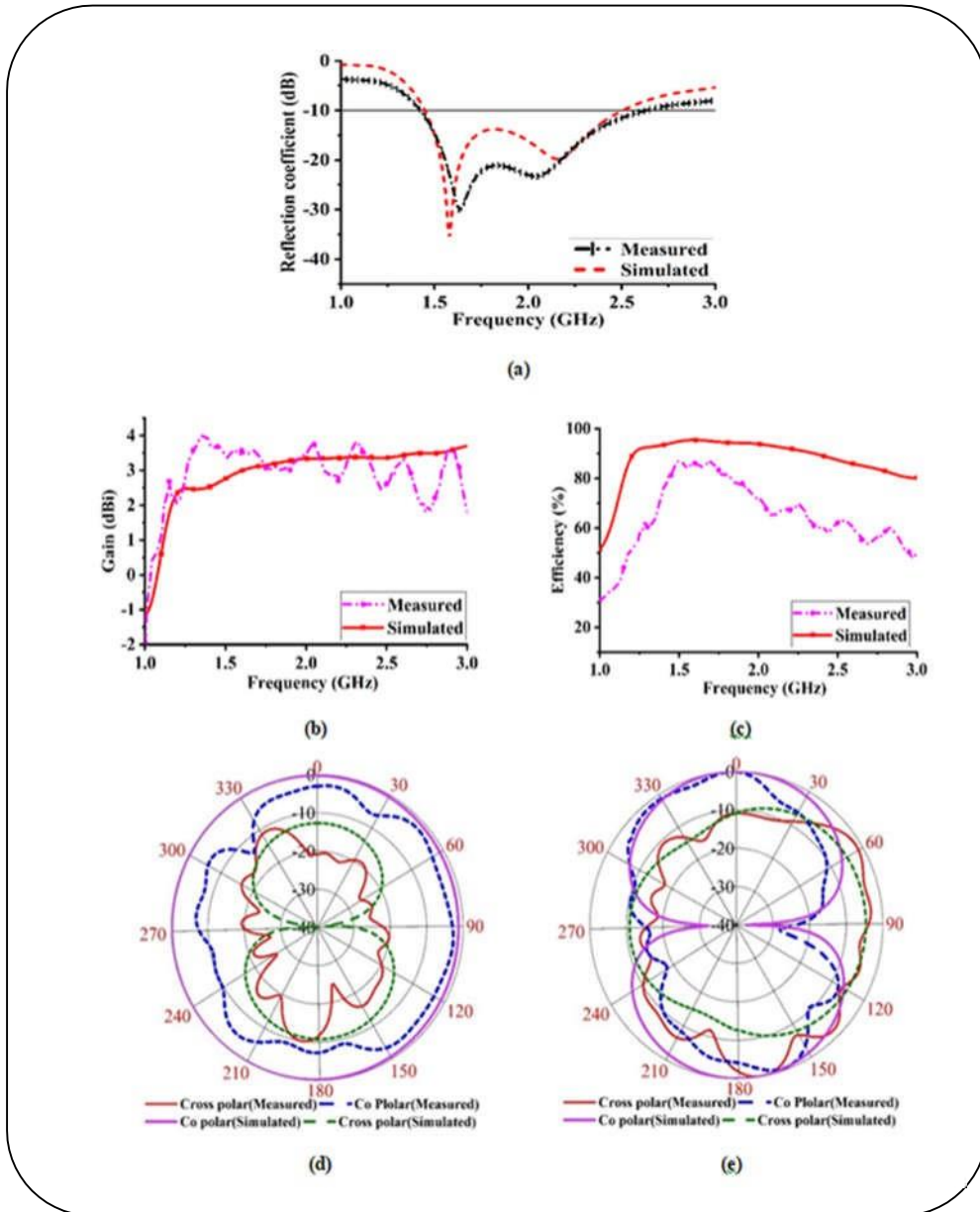
Figure 5. Measured antenna properties; (a) Reflection coefficient, (b) max gain(dBi), (c) radiation efficiency (%), (d) radiation pattern at 1.58 GHz along xz-plane, (e) radiation pattern at 1.58 GHz along yz-plane.
