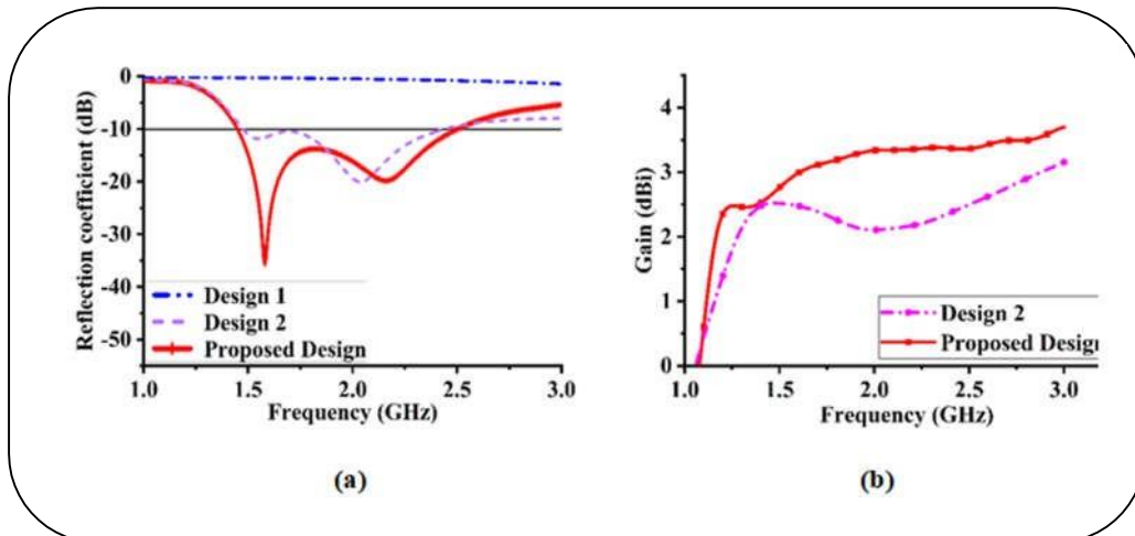
Figure 2. Antenna Performance in Each Step of Try and Error Method; (a) Reflection Coefficient; (b) Gain.
